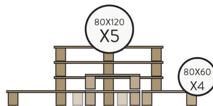
PALETS (PROFILE VIEW)
